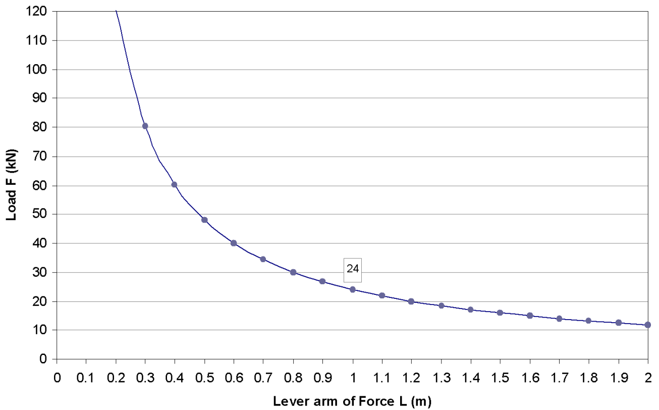
Load diagram for rotator CPR 8 series
